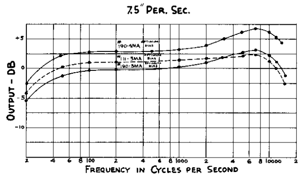
FIG. 1 FREQUENCY RESPONSE OF #190 TAPE
